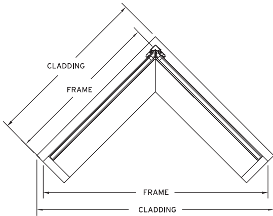
Interior Glazed Unit Standard Side Jamb (top view)
